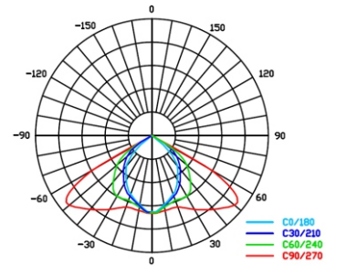
Light Diagram
